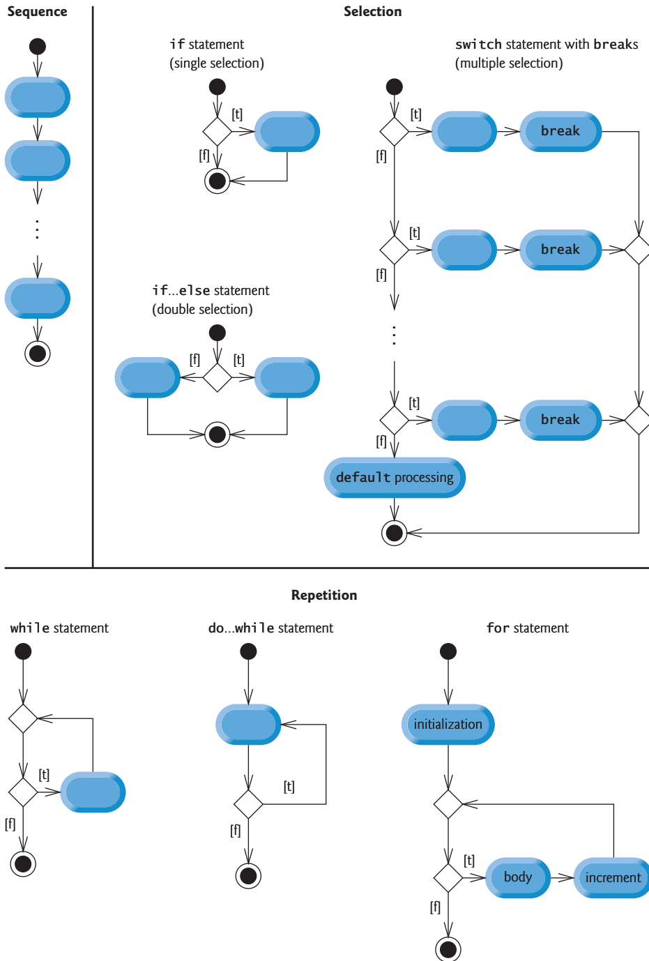
Fig. 5.20 | C++'s single-entry/single-exit sequence, selection and repetition statements.
