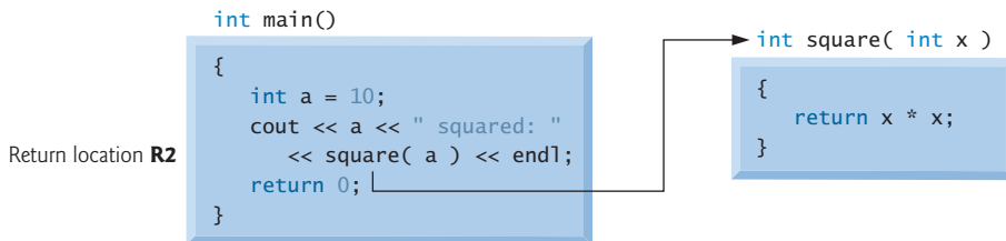
Fig. 6.15 | Function call stack after main invokes square to perform the calculation. (Part 1 of 2.)
