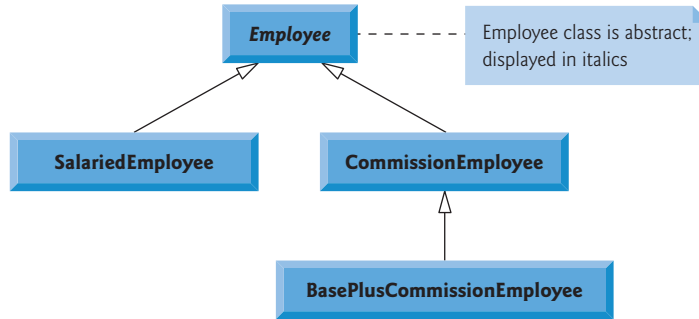
Fig. 13.7 | Employee hierarchy UML class diagram.
