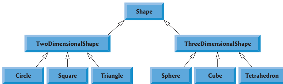
Fig. 12.3 | Inheritance hierarchy for Shapes.
