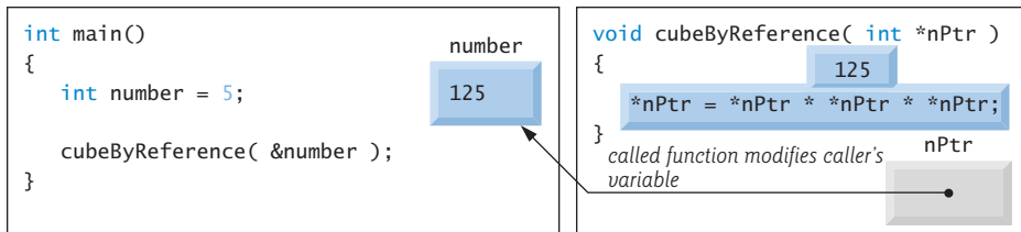
Fig. 8.9 | Pass-by-reference analysis (with a pointer argument) of the program of Fig. 8.7.
